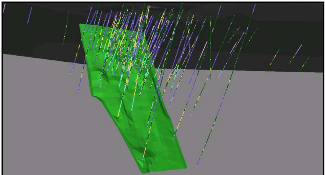
Figure 7.7 Zone 5 Oblique Long Section (not to scale)
