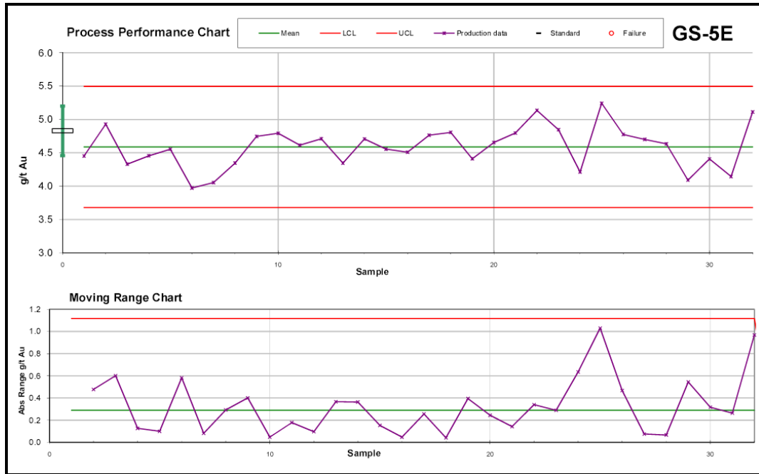
Figure 11.4 GS-5E Process Performance Chart
