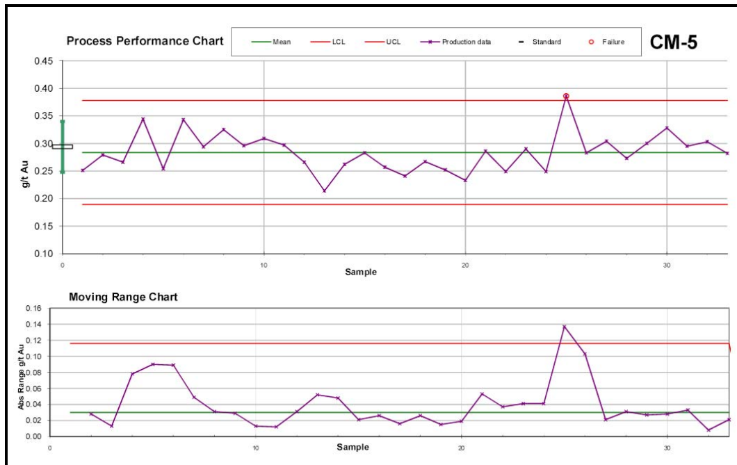
Figure 11.2 CM-5 Process Performance Chart
