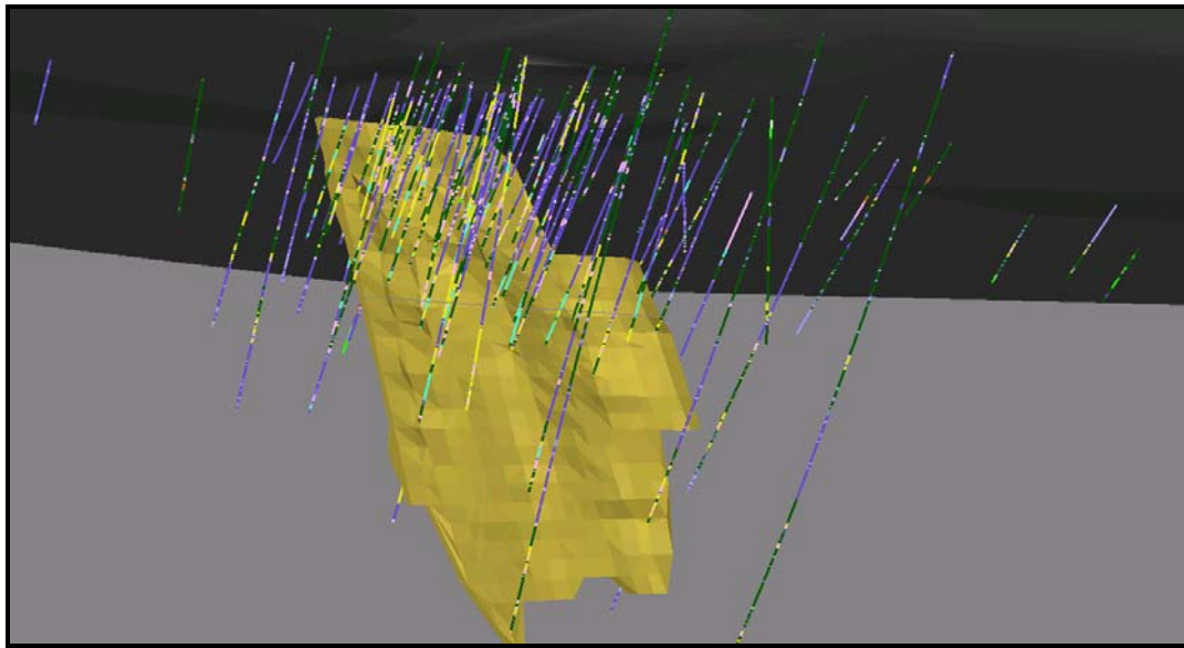
Figure 7.5 Zone 3 Oblique Long Section (not to scale)
