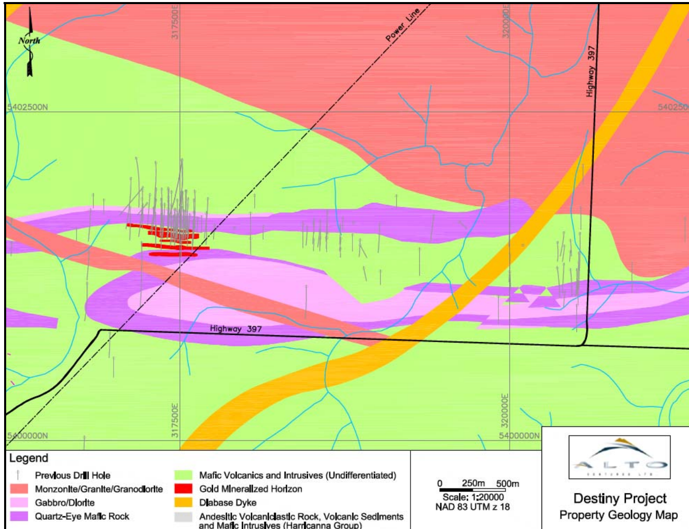
Figure 7.2 Property Geology
