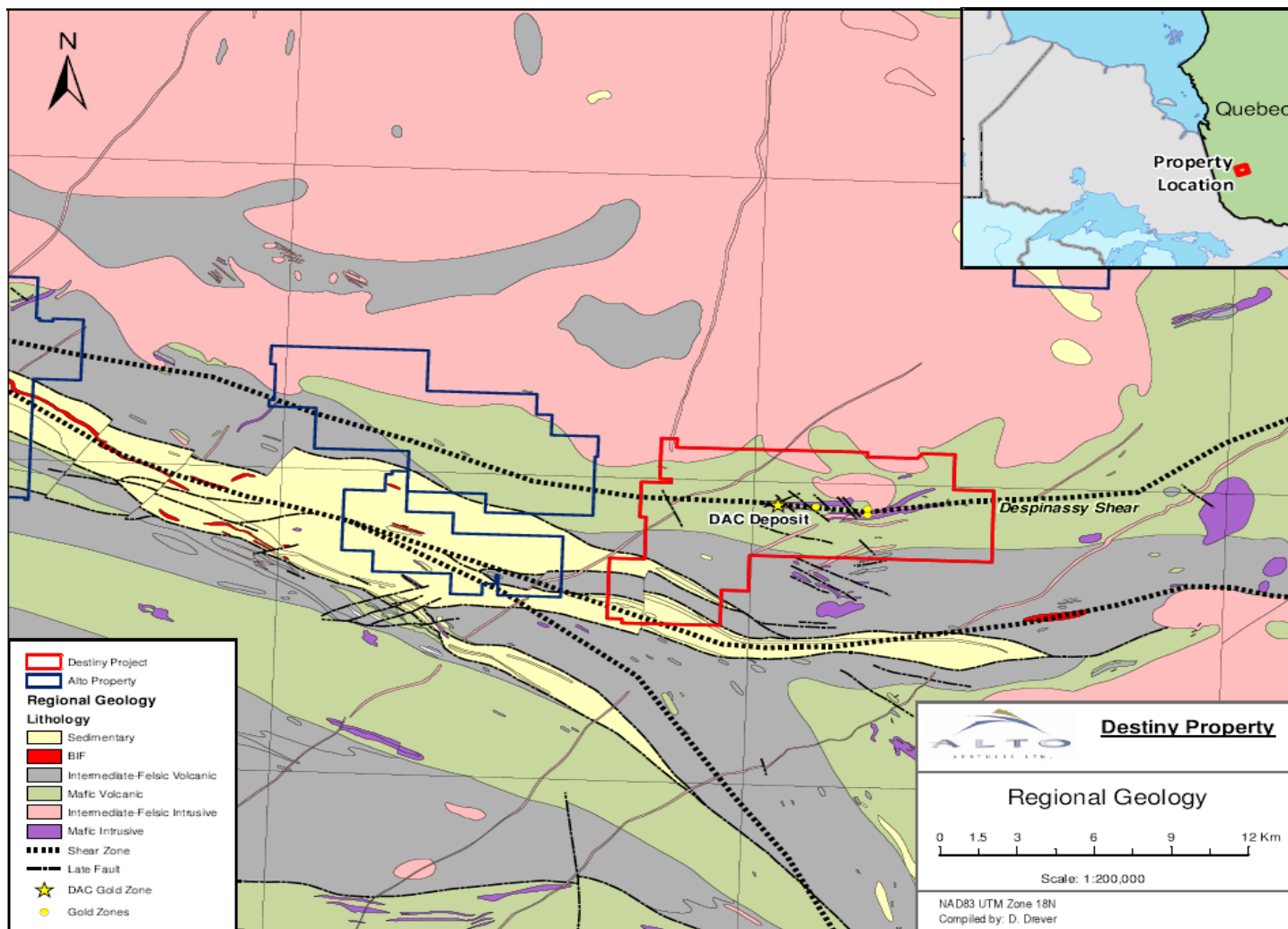
Figure 7.1 Regional Geology
