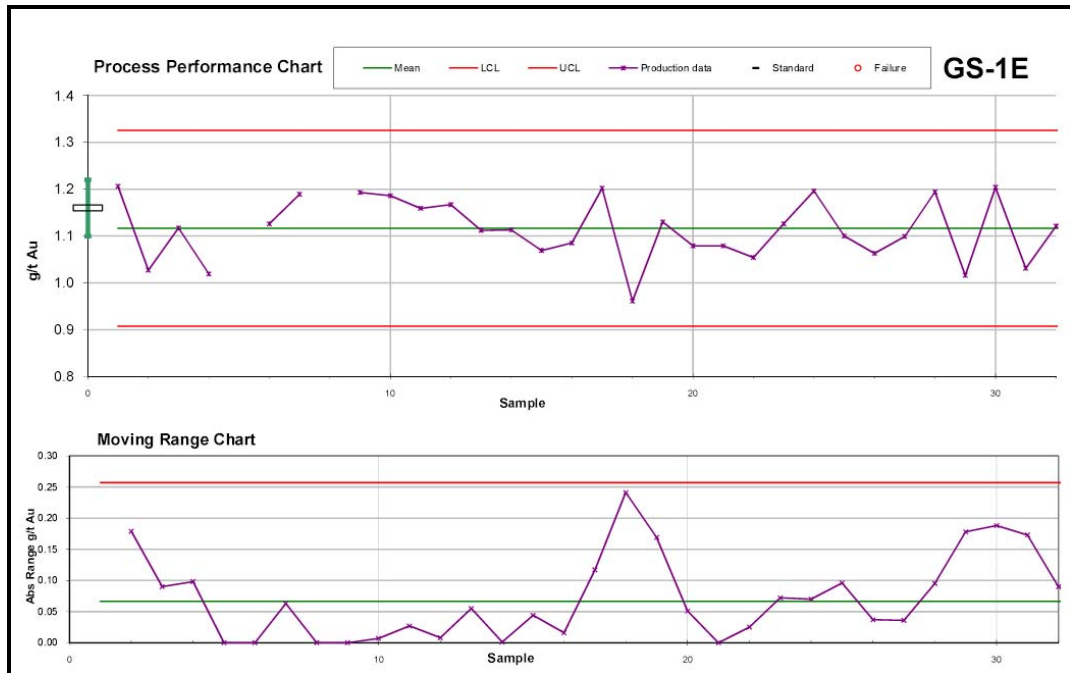
Figure 11.3 GS-1E Process Performance Chart
